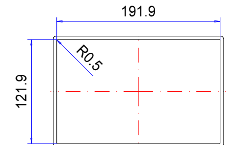
Keypad 121.3 +0 -0.2 x 191.3 +0 -0.2
