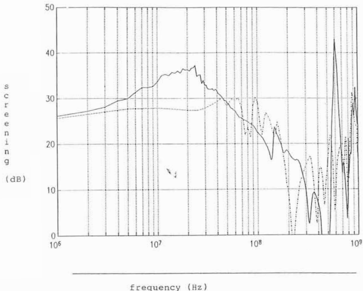
Fig. 3.1: Comparison of the results of the two measuring methods, illustrated using the example of a casing of the older type
