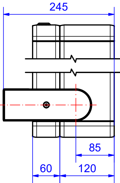
profiles 120-60
