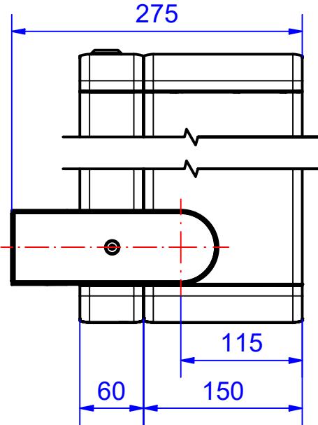
profiles 150-60
