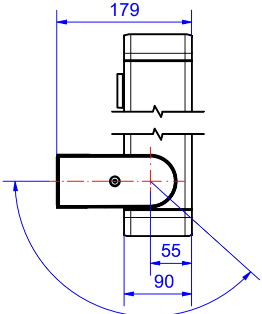
profile depth 90mm
