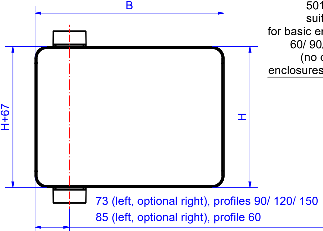
profile depth 60mm
