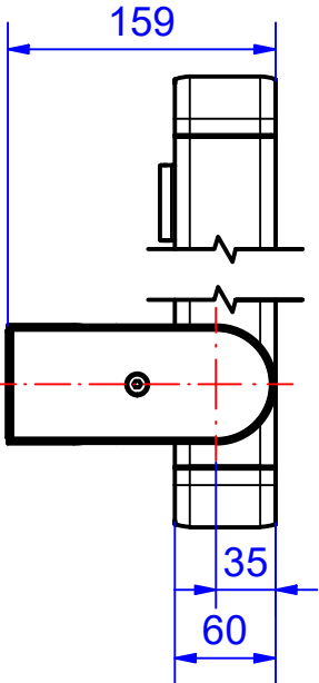
profile depth 60mm
