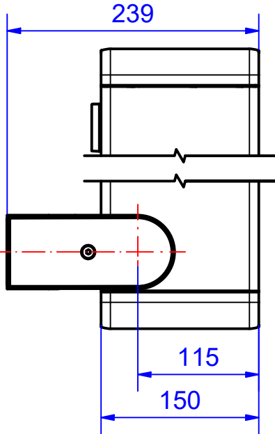
profile depth 150mm
